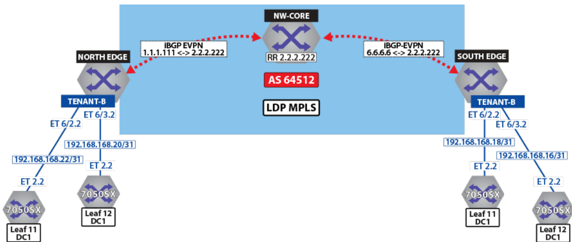
Figure 127: Control Plane Tenant-B over LDP
