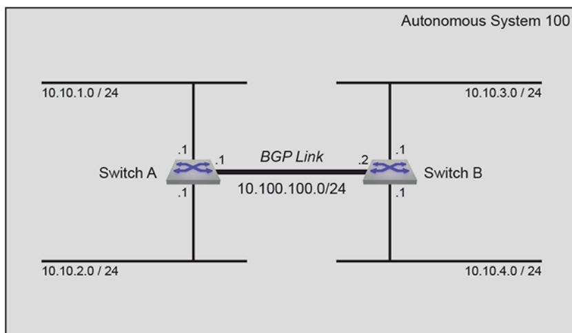
Figure 60: BGP Example 1
