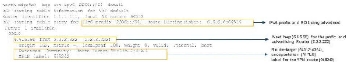
Figure 98: IPv6 VPN Route as Shown on PE
