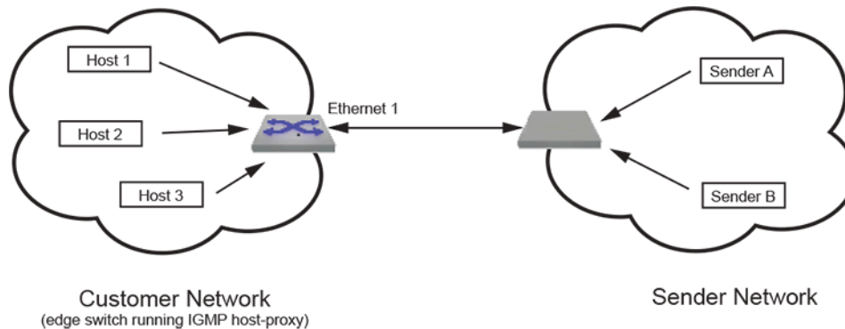
Figure 65: IP IGMP Host Proxy Implementation
