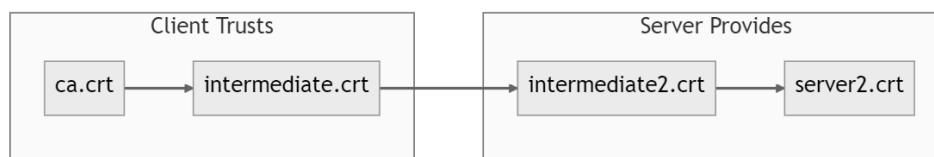
Figure 4: Certificate Chain Example 2
