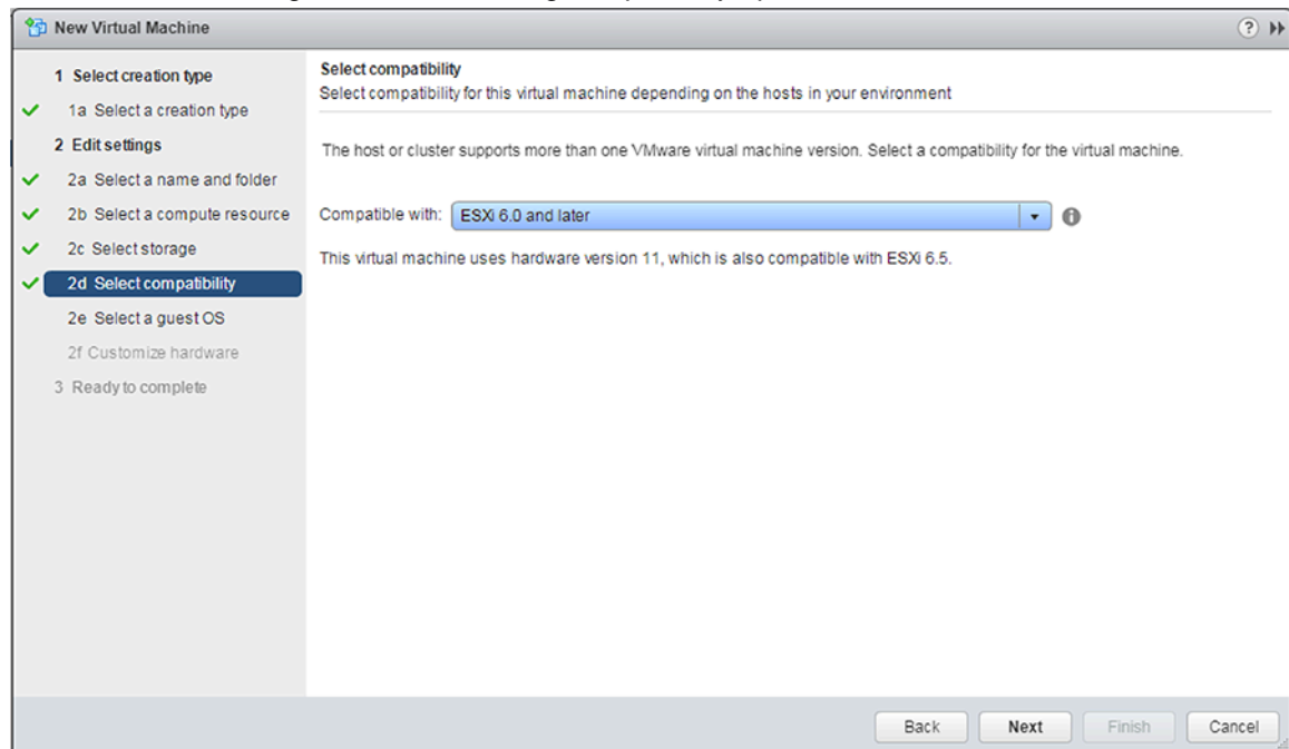
Figure 42: New Virtual Machine Dialog (Compatibility Options)
