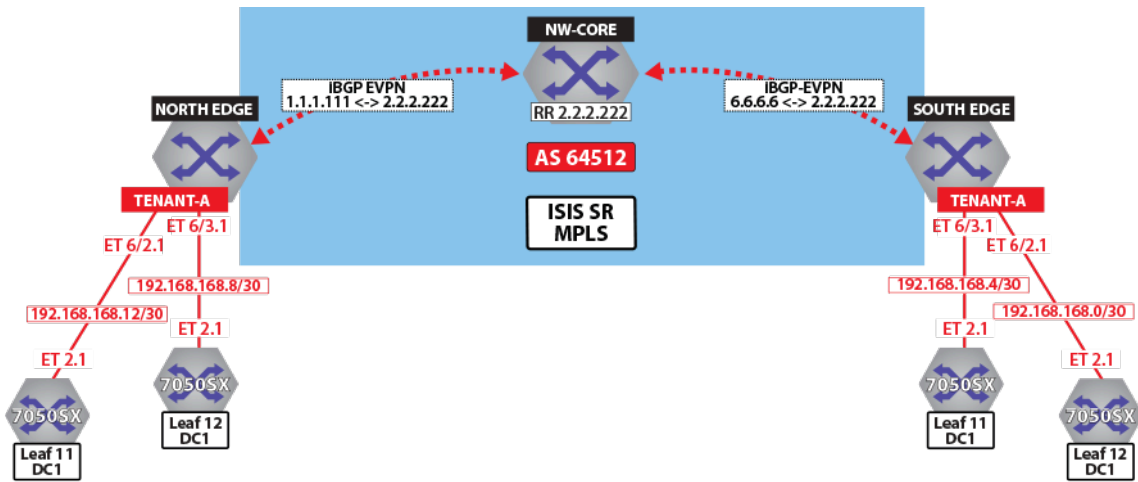
Figure 126: Control Plane Tenant-A Over LDP
