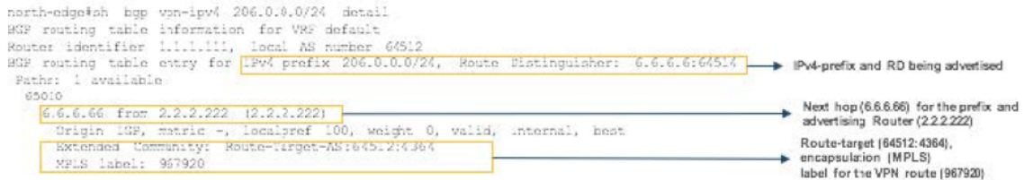
Figure 97: IPv4 VPN Route as Shown on PE
