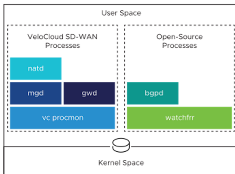
Figure 2-1: SD-WAN Gateway Overview
