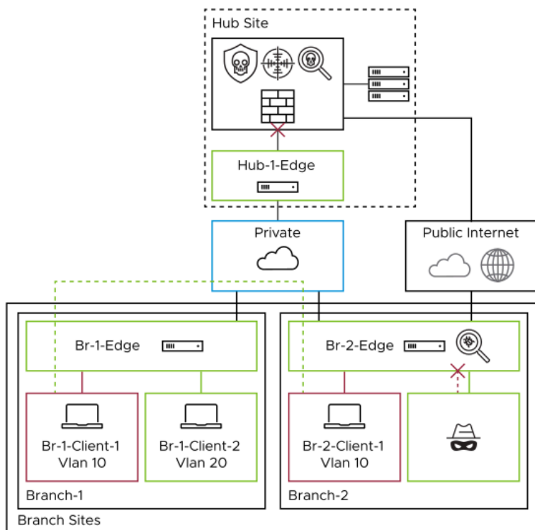
Figure 5-1: Inter-Branch Communication
