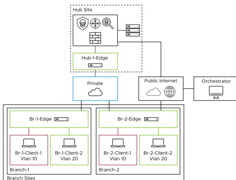
Figure 3-1: Topology Diagram
