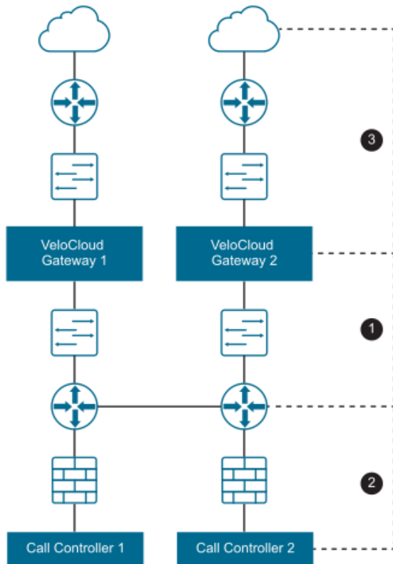
Figure 14-13: SD-WAN Gateway topology
