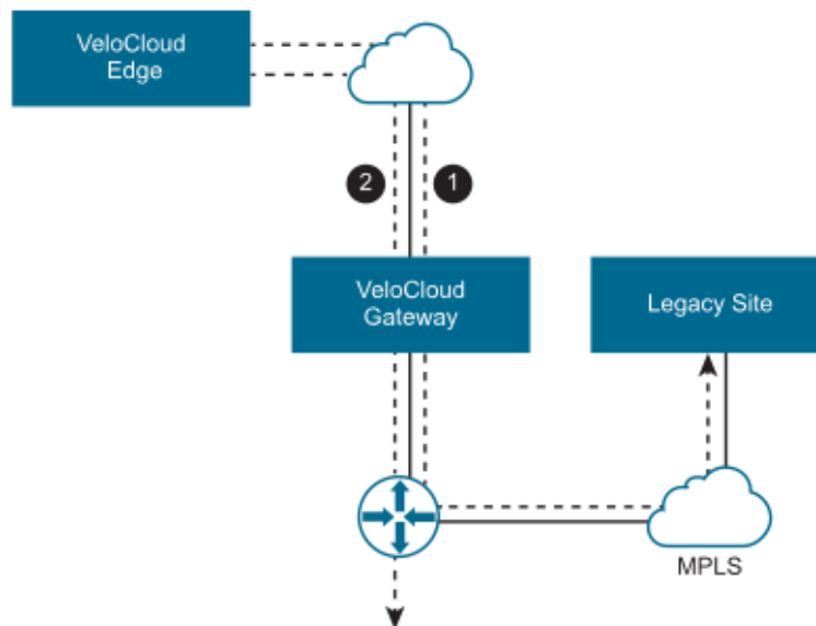
Figure 14-12: Partner Gateway Configuration Use Case 2
