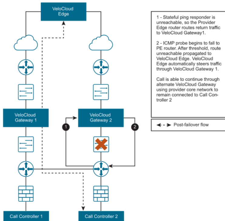
Figure 14-14: Failure Scenario between SD-WAN Gateway and Edge
