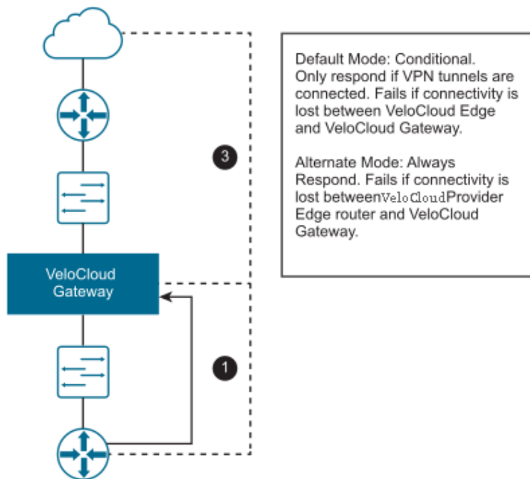
Figure 14-15: Stateful Ping Responder Scenario
