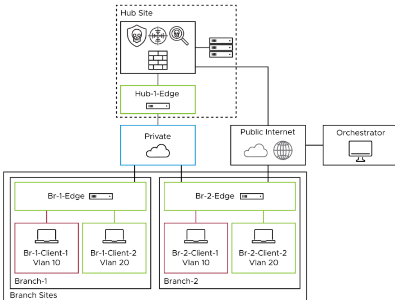
Figure 3-1: Topology Diagram
