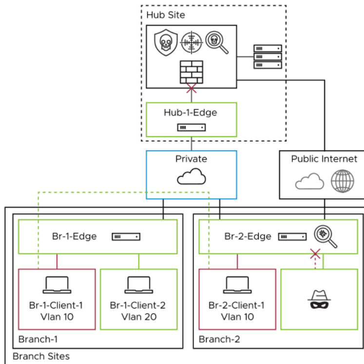
Figure 5-1: Inter-Branch Communication
