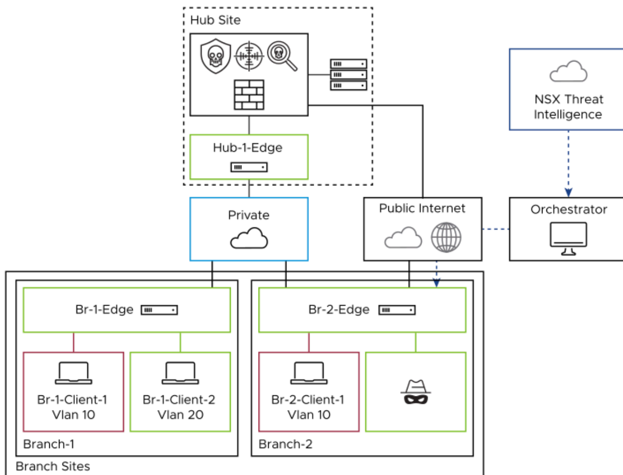
Figure 3-2: Signature Flow Diagram
