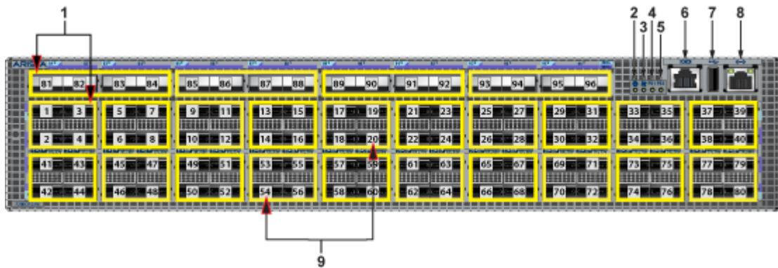
Figure C-15: DCS-7280CR3-96
