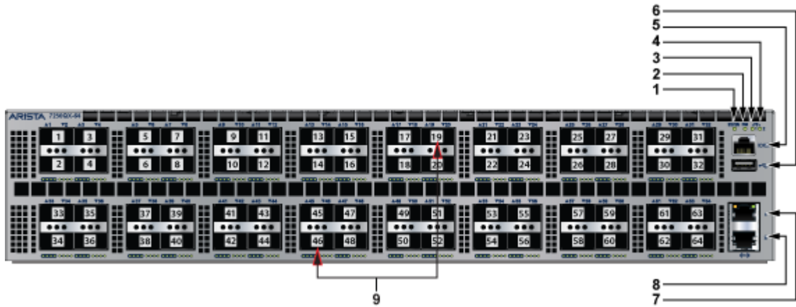
Figure C-5: DCS-7250QX-64
