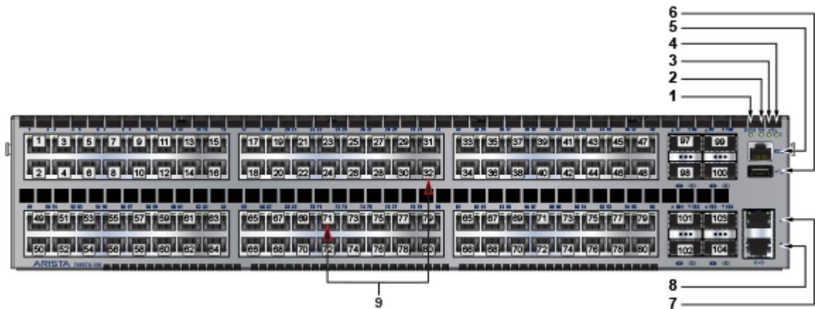
Figure C-2: DCS-7050TX-128
