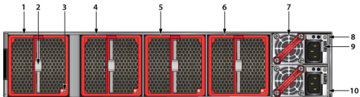
Figure D-3: Models with separation between Fans 1 and 2 (no ground)
