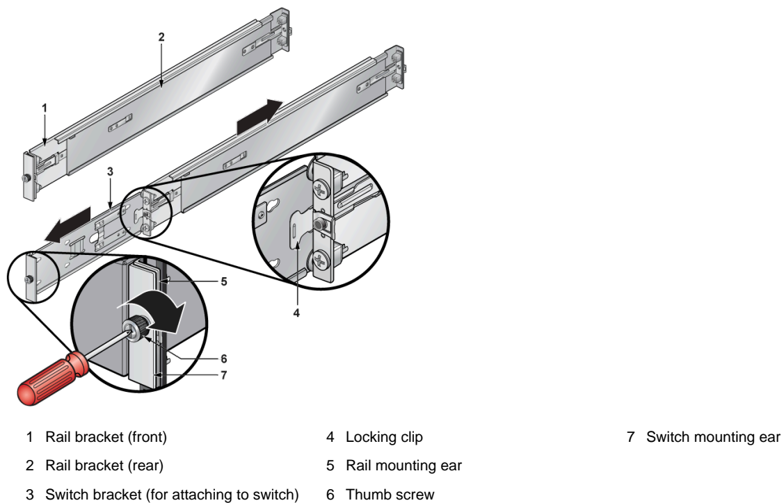
Figure 3-11: Accessory Kit Components
