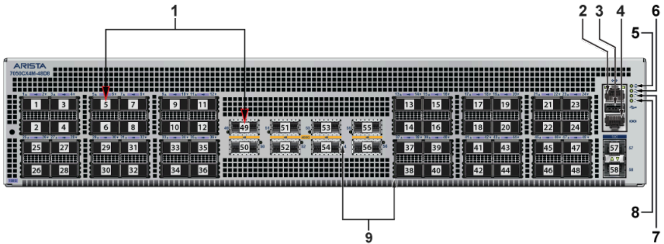
Figure C-7: DCS-7050CX4M-48D8
