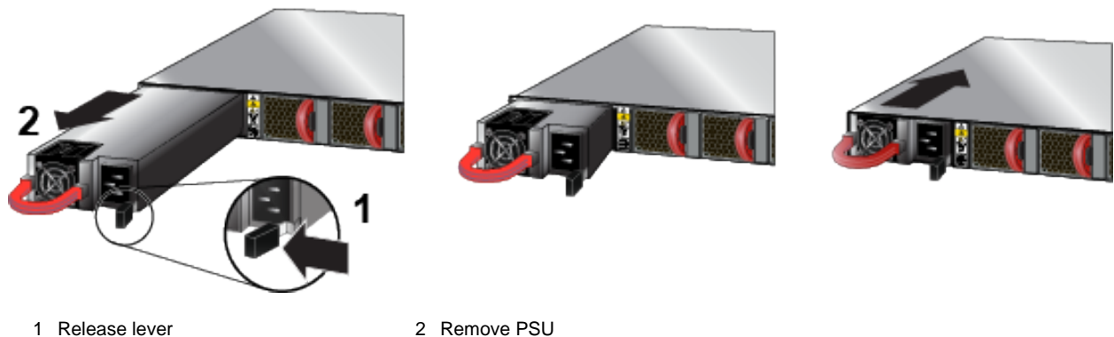
Figure E-1: Removing and Installing Power Supply
