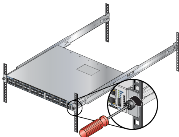
Figure 3-10: Attaching the Switch to the Rack Posts
