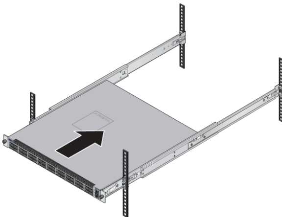
Figure 3-9: Inserting the Switch onto the Rails
