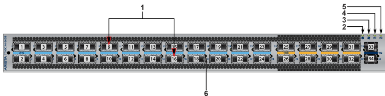
Figure C-5: DCS-7050CX4-24D8
