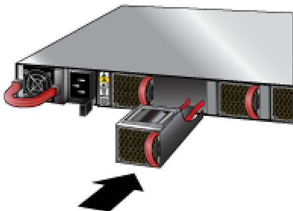
Figure E-3: Inserting Fan Module
