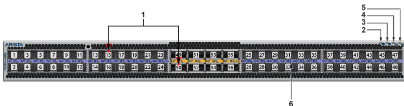
Figure C-4: DCS-7050SPX4-48D8
