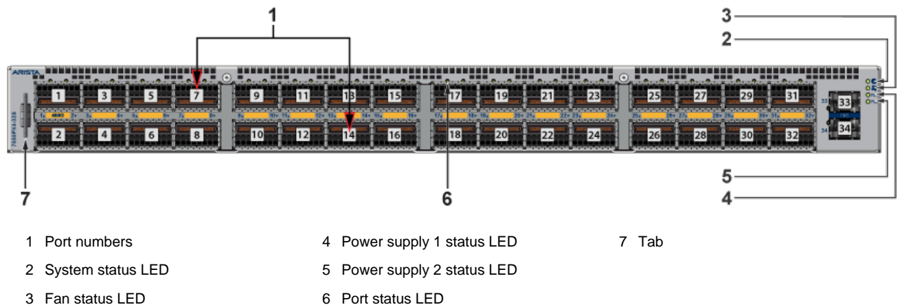
Figure C-2: DCS-7050PX4-32S
