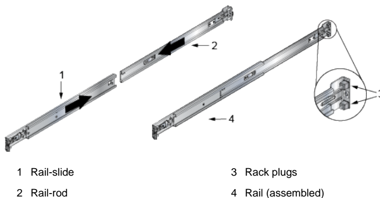
Figure 3-7: Assembling the Rails
