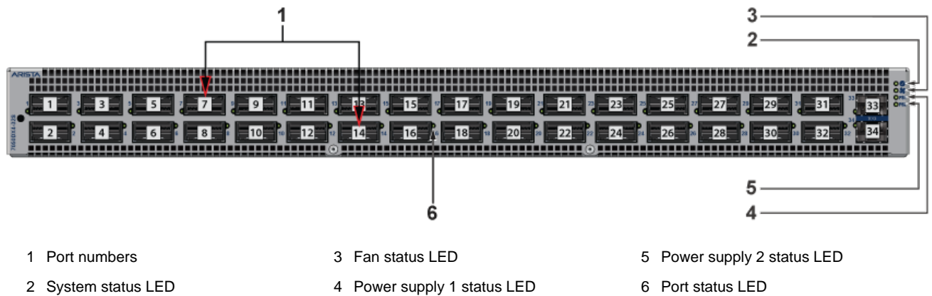
Figure C-1: DCS-7050DX4-32S and DCS-7050DX4M-32S
