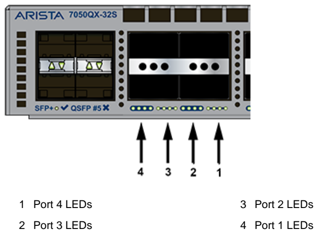
Figure A-2: Port LEDs
