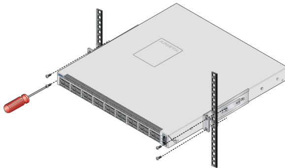
Figure 3-3: Inserting the Switch into the Rack
