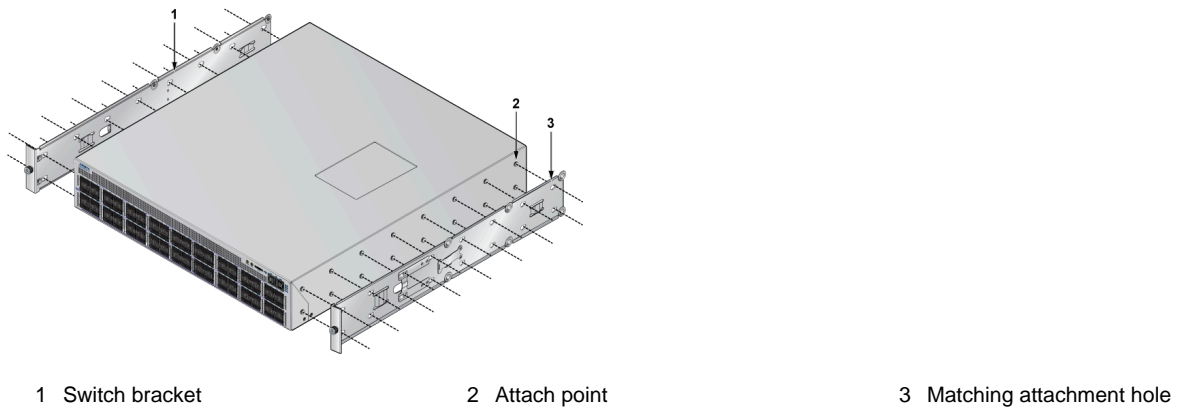
Figure 3-12: Front Bracket Alignment
