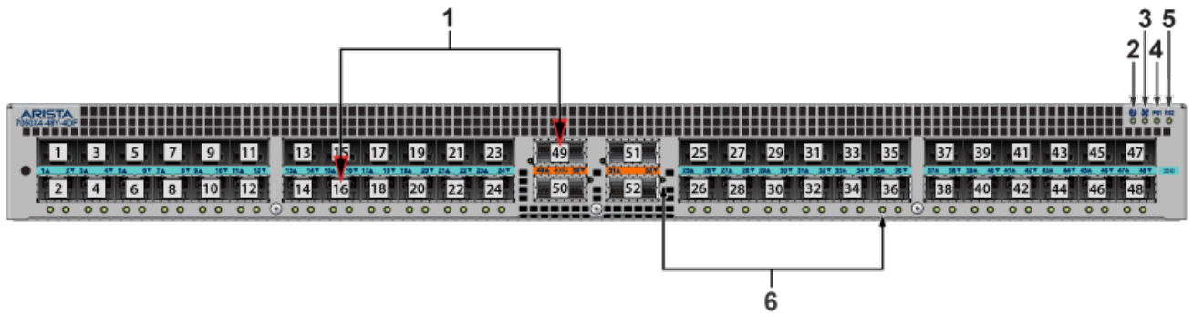
Figure C-6: DCS-7050X4-48Y-4DF
