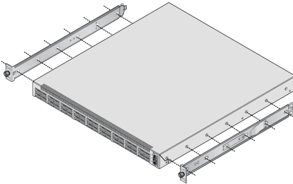
Figure 3-5: Attaching the Mounting Brackets to the Switch Chassis (with Deep Chassis Adapters)
