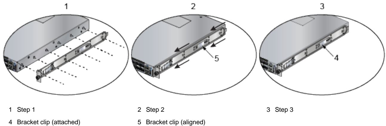
Figure 3-6: Attaching the Four-Post Mounting Brackets to the Switch Chassis
