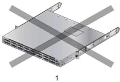
Figure 3-5: Improper Bracket Mount Configuration for Four-Post Rack Mount (Example)
