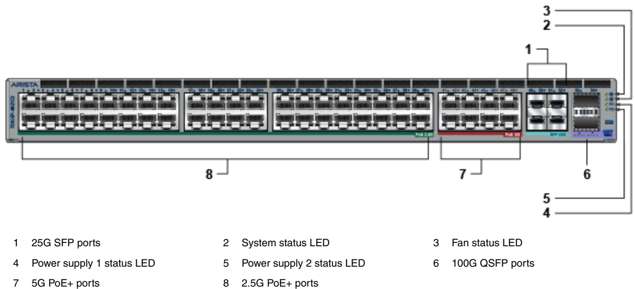
Figure A-1: System Status Indicators
