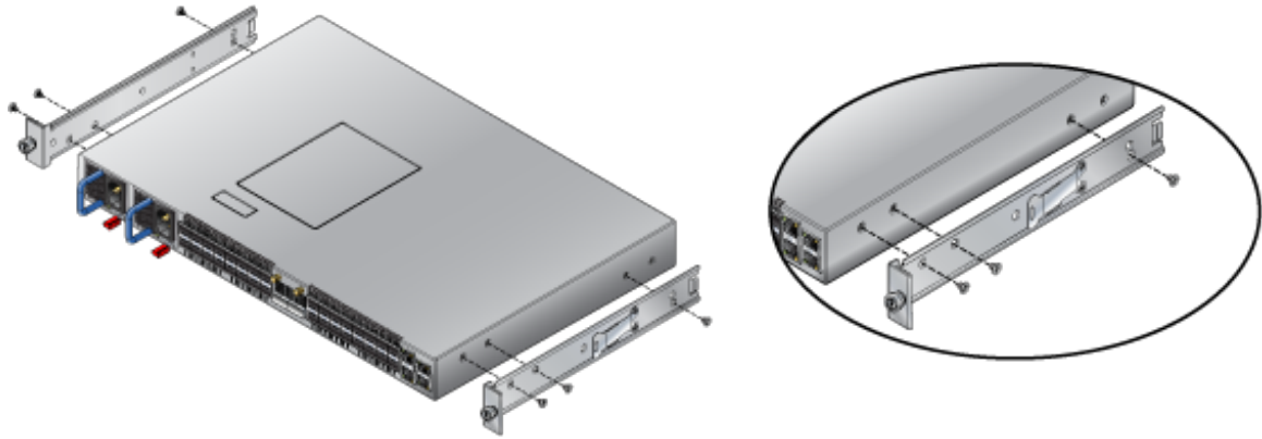
Figure 3-2: Attaching Mounting Brackets to the Switch Chassis
