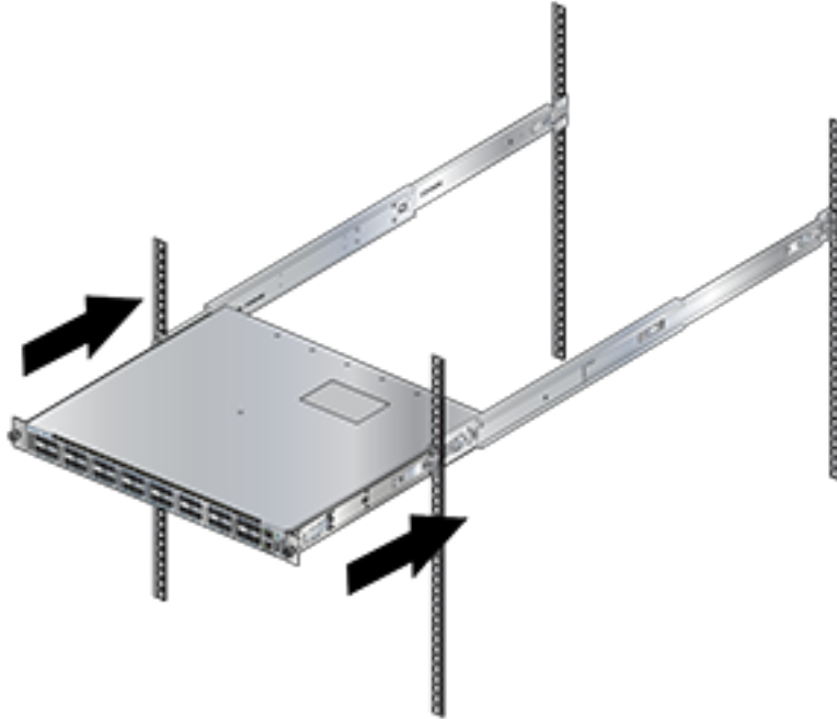
Figure 3-10: Inserting the Switch onto the Rails
