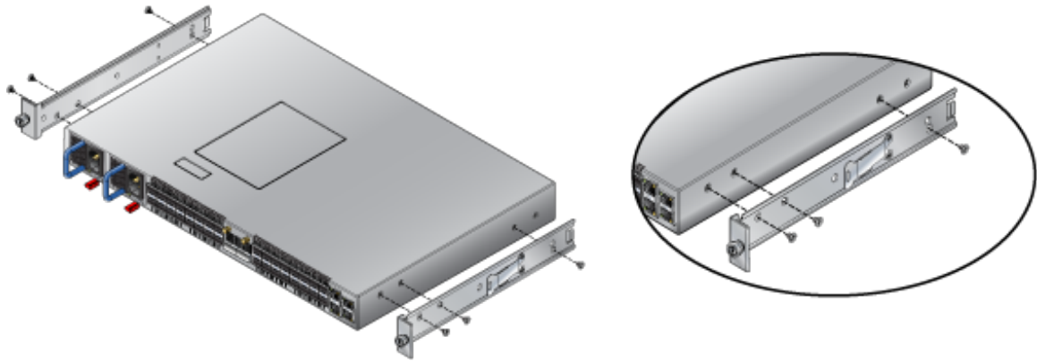
Figure 3-6: Attaching Mounting Brackets to the Switch Chassis
