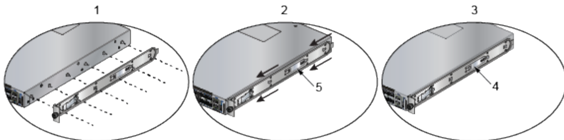
Figure 3-7: Attaching the Mounting Brackets to the Switch Chassis
