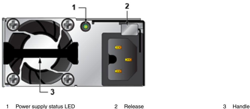
Figure 4-2: AC Power Supply (PWR-1021-AC-RED)
