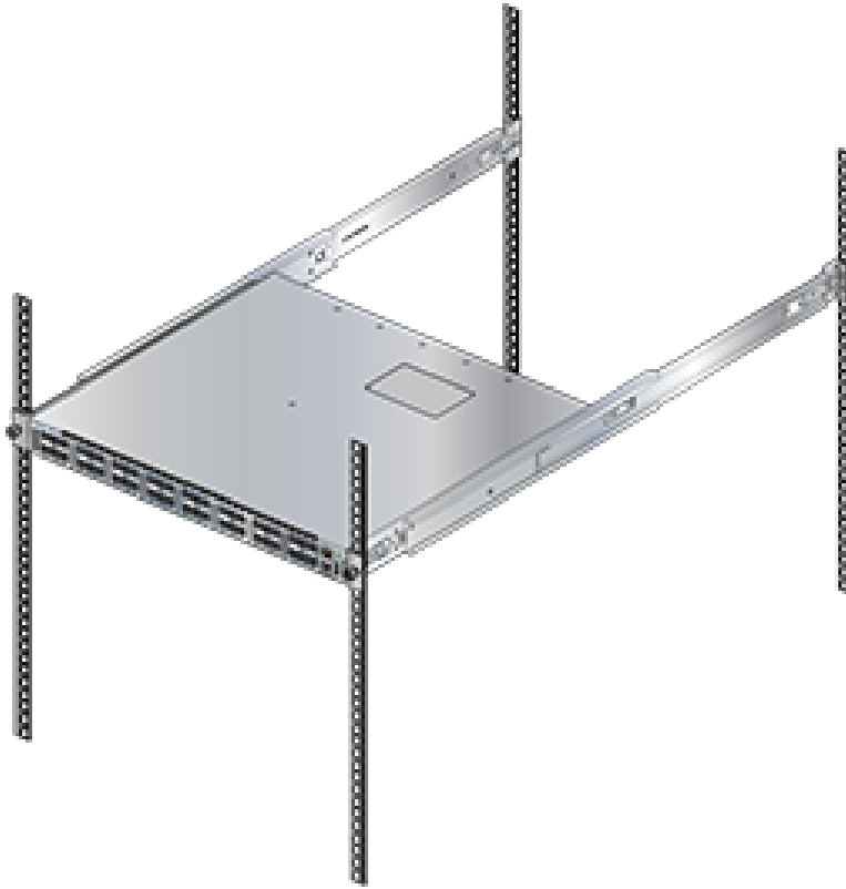
Figure 3-11: Attaching the Switch to the Rack Posts
