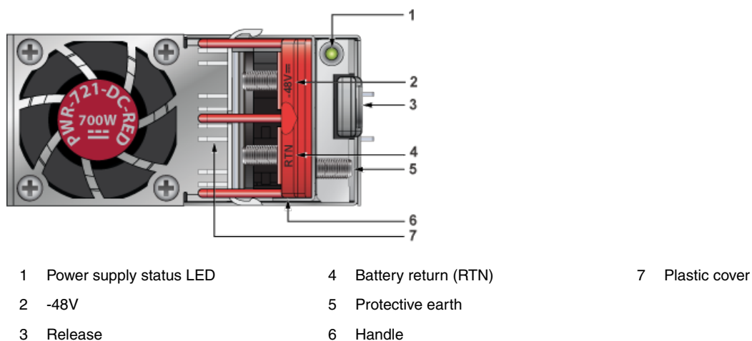
Figure 4-3: DC Power Supply (PWR-721-DC-RED)
