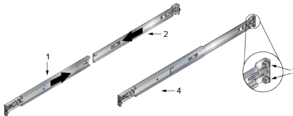
Figure B-2: Four-Post Rack Mounting Parts
