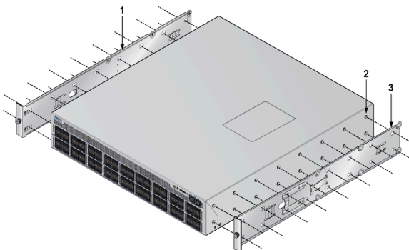
Figure 3-15: Front Bracket Alignment
