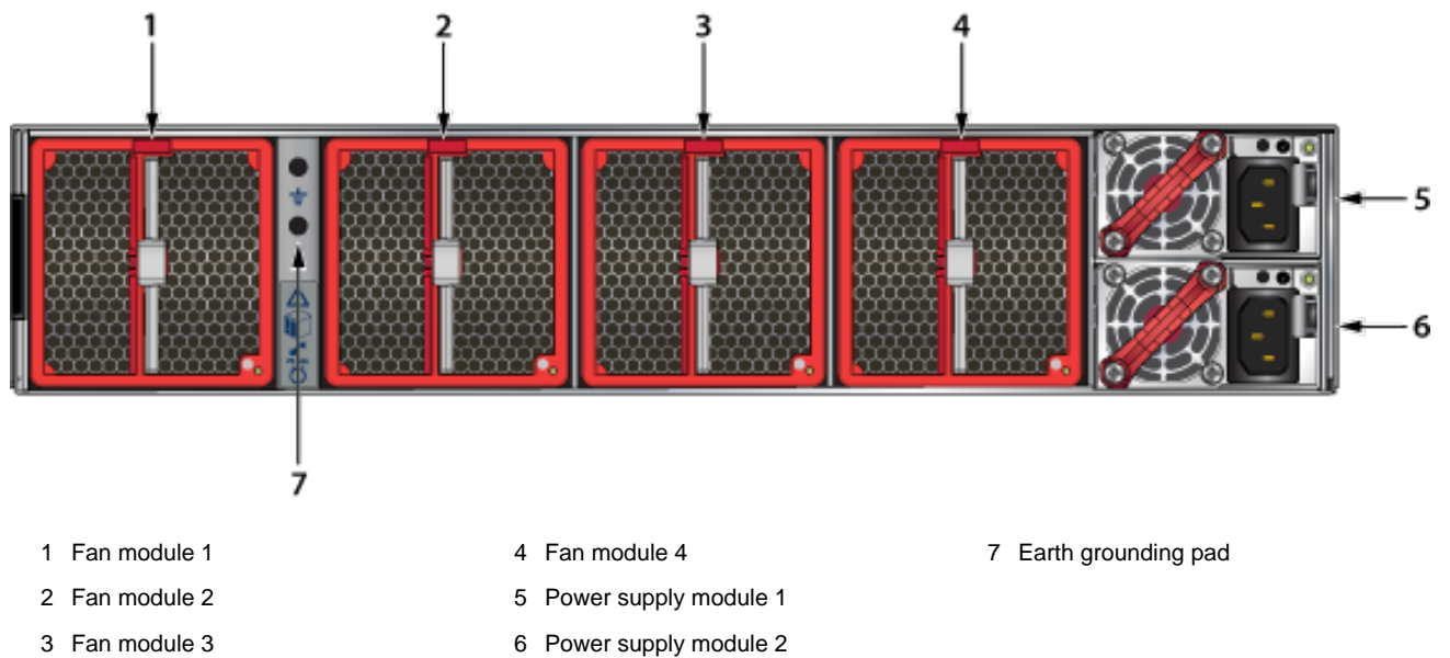
Figure D-3: Rear Panel with Ground Attach Point (2RU)
