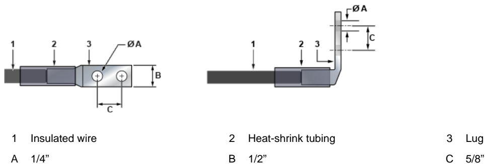
Figure 4-6: Lug Preparation
