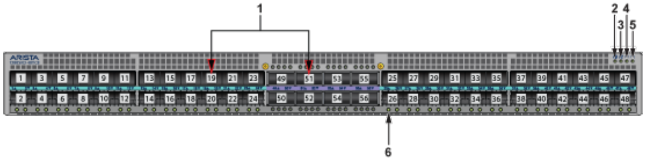
Figure C-6: DCS-7280SR3-48YC8, DCS-7280SR3K-48YC8, and DCS-7280SR3K-48YC8A
