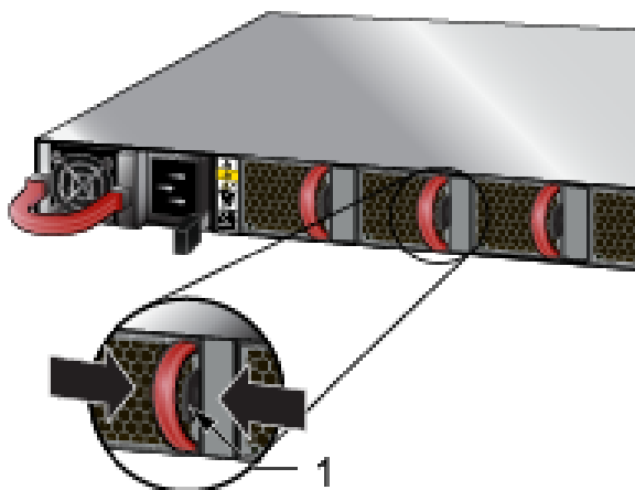
Figure E-2: Removing a Fan Module
