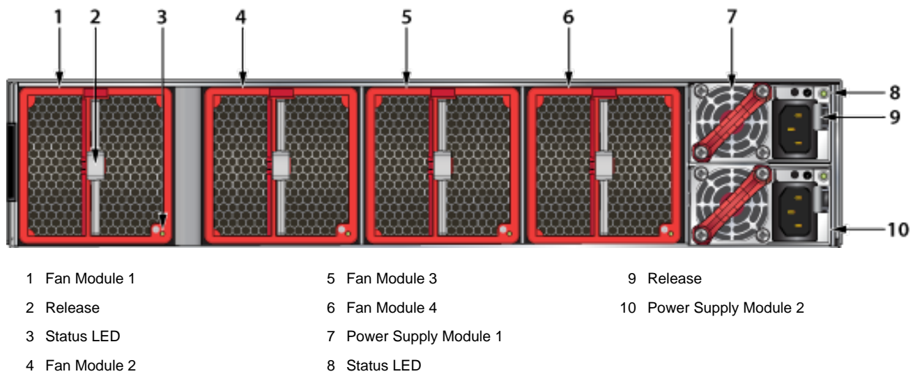
Figure D-4: Rear Panel with Separation Between Fans 1 and 2 (no ground)
