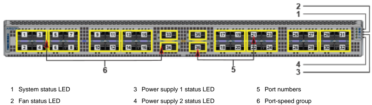
Figure C-4: DCS-7280CR3-32D4, 7280CR3K-32D4, and DCS-7280CR3K-32D4A
