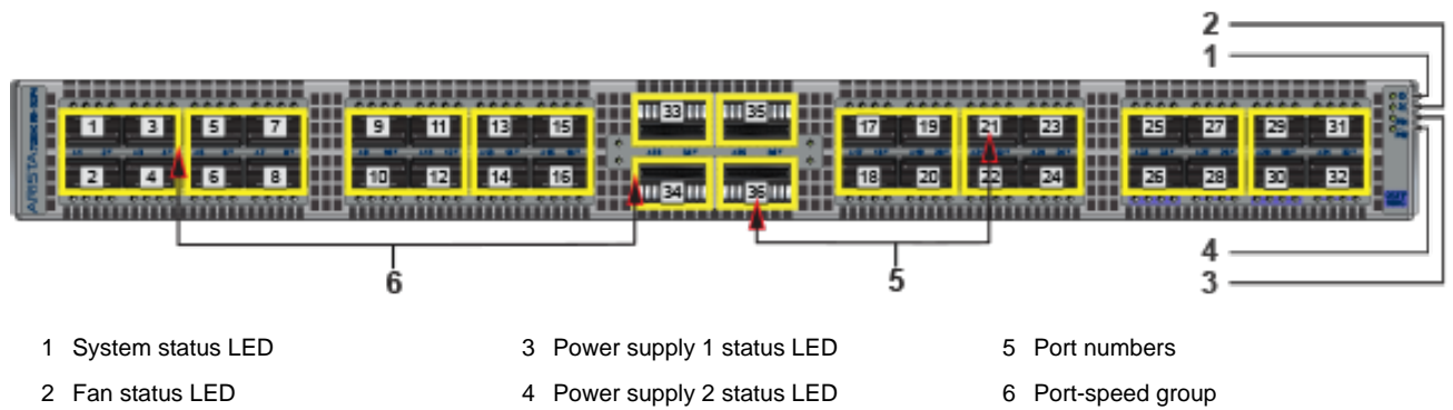
Figure C-3: DCS-7280CR3-32P4, DCS-7280CR3K-32P4, and DCS-7280CR3K-32P4A
