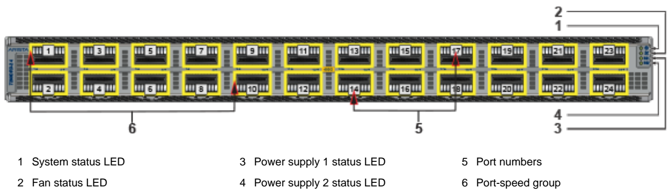
Figure C-2: DCS-7280DR3-24 and DCS-7280DR3K-24
