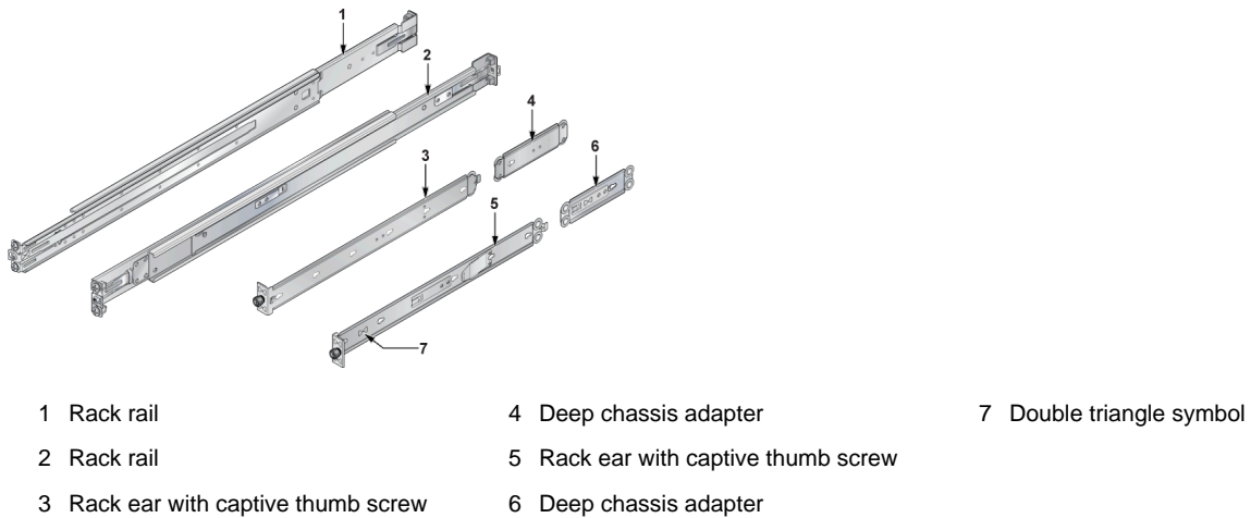
Figure B-3: Four-Post Rack Mounting Brackets with Roller Extensions
