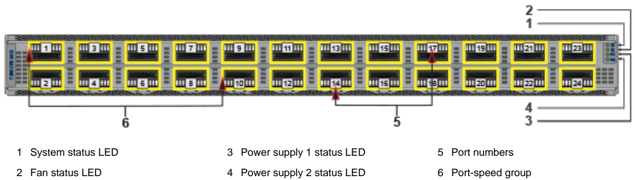
Figure C-1: DCS-7280PR3-24 and DCS-7280PR3K-24
