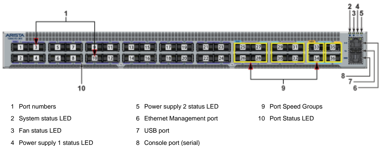
Figure C-5: DCS-7280CR3-36S, DCS-7280CR3K-36S, and DCS-7280CR3K-36A
