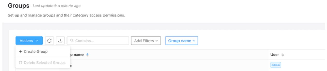
Figure 11-17: Group Creation
