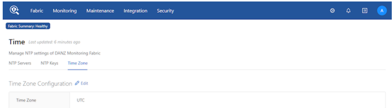
Figure 2-6: Time Zone
