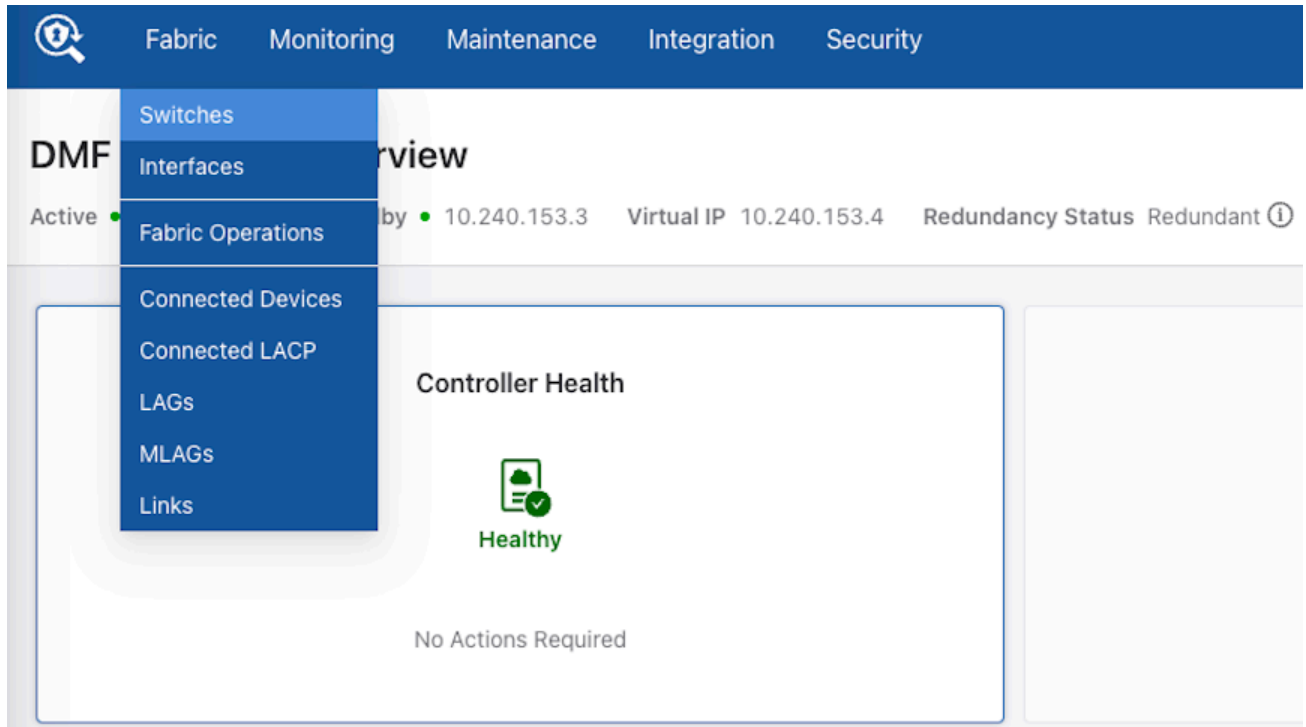
Figure 4-17: Fabric > Switches
