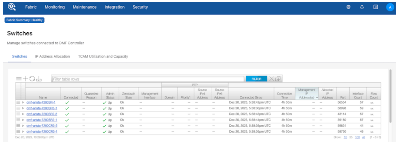
Figure 4-18: Switches
