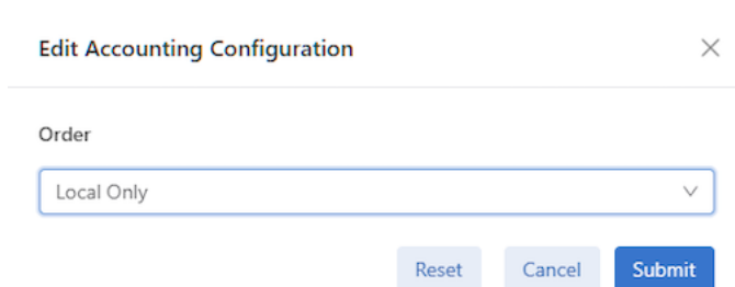
Figure 11-9: Accounting Settings
