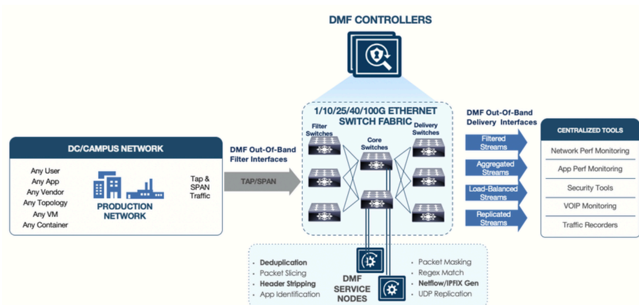
Figure 7-1: DMF Service Node
