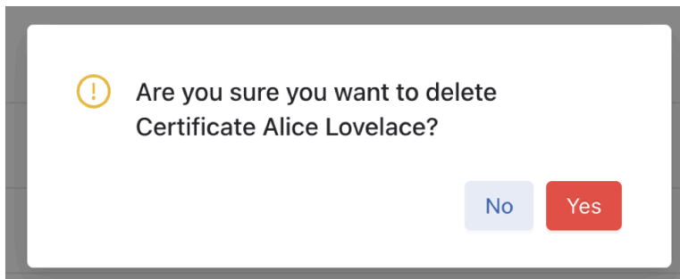
Figure 12-5: Confirmation Window
