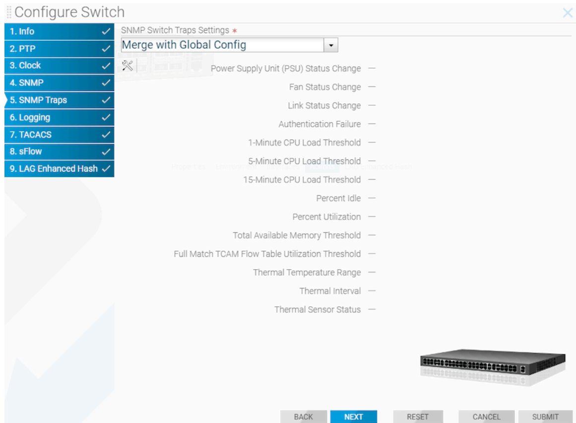
Figure 10-27: SNMP Traps
