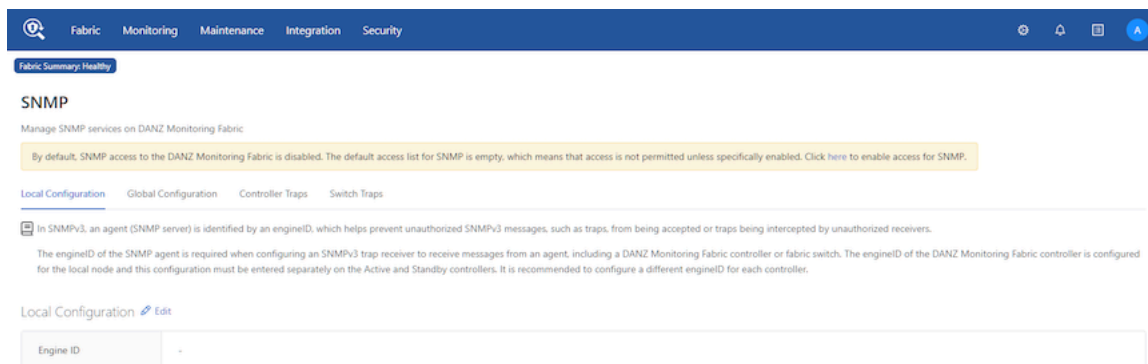
Figure 10-1: Configuring SNMP
