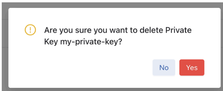
Figure 12-11: Confirmation Window
