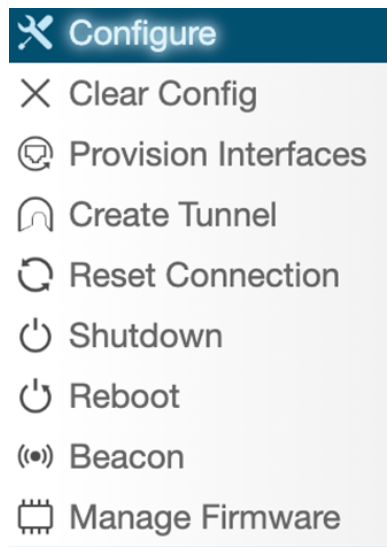
Figure 4-9: Configure
