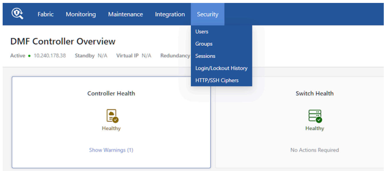
Figure 11-1: Security
