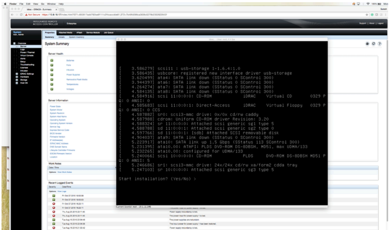
Figure 13-33: Installation Prompt
