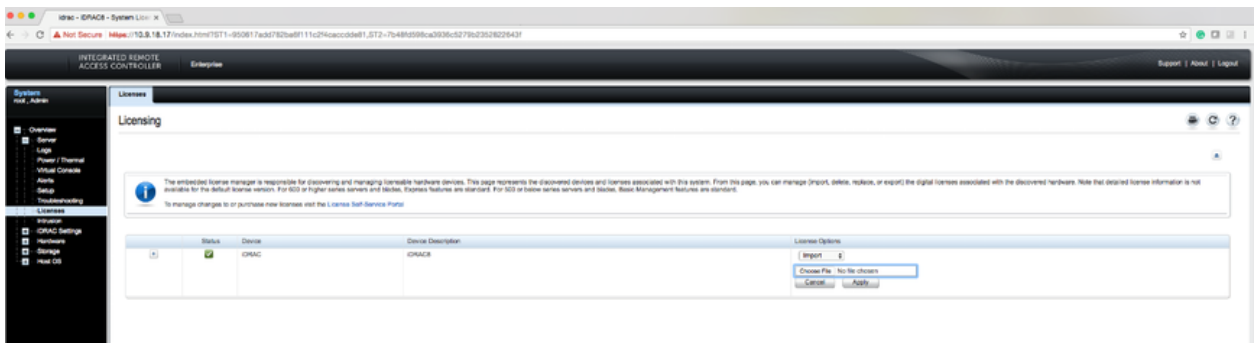
Figure 13-9: Licensing Page
