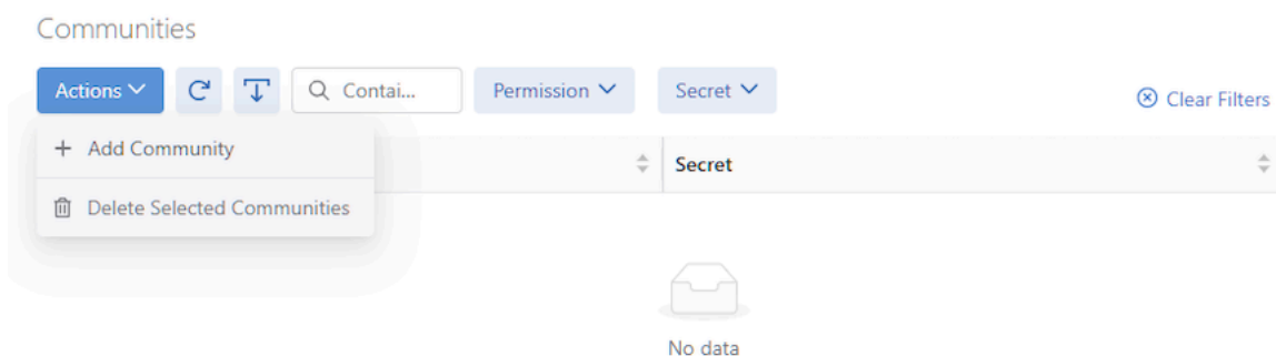
Figure 10-10: Add Community
