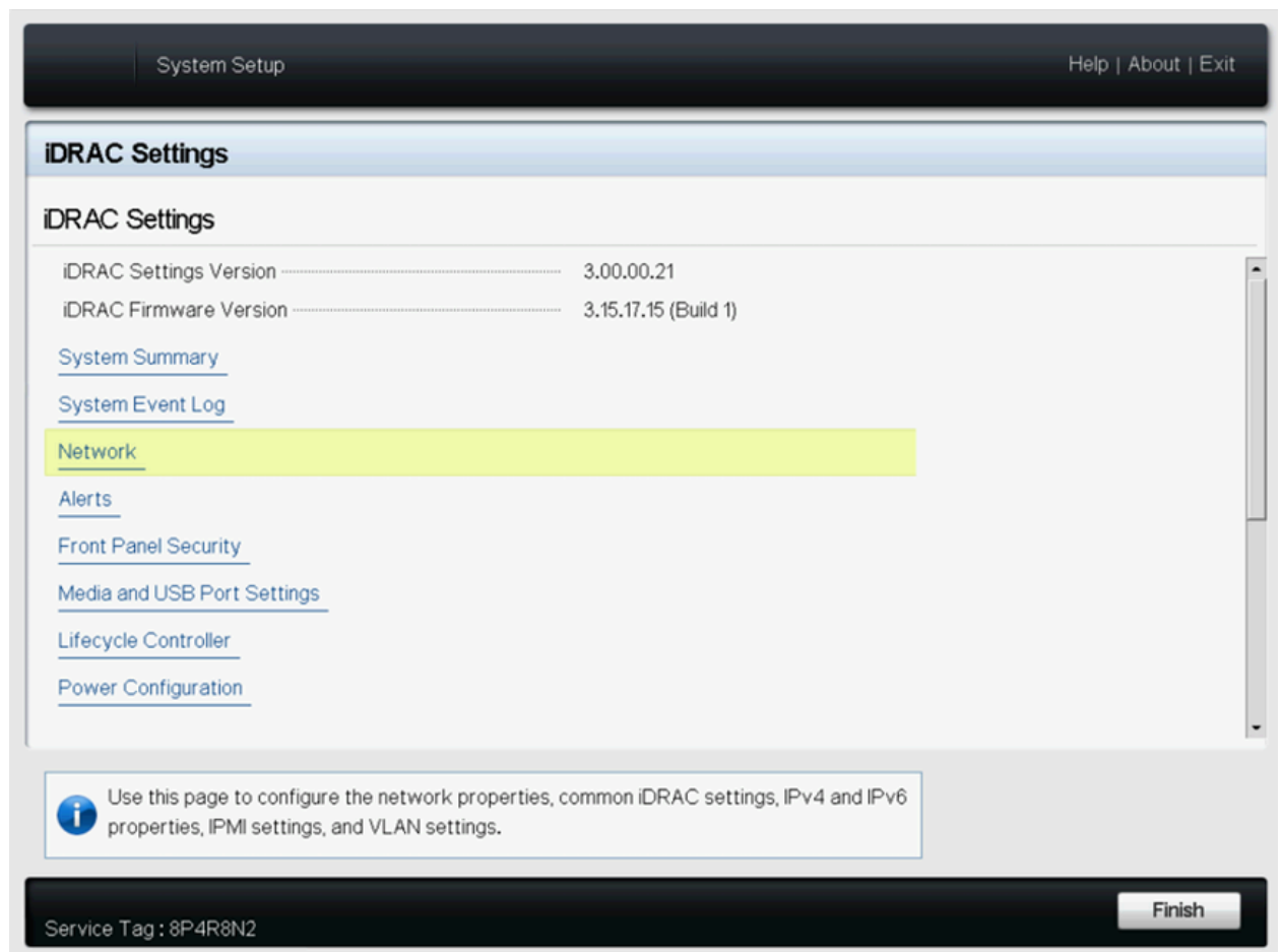
Figure 14-2: iDRAC Settings
