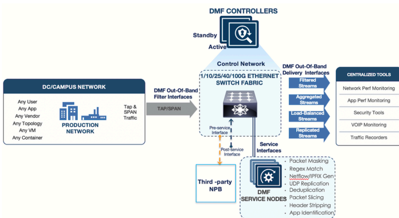
Figure 3-1: DANZ Monitoring Fabric (DMF) Single Switch Topology
