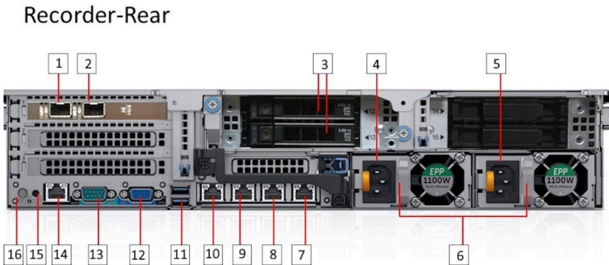
Figure 8-3: DMF Recorder Node (HWA) Rear Panel
