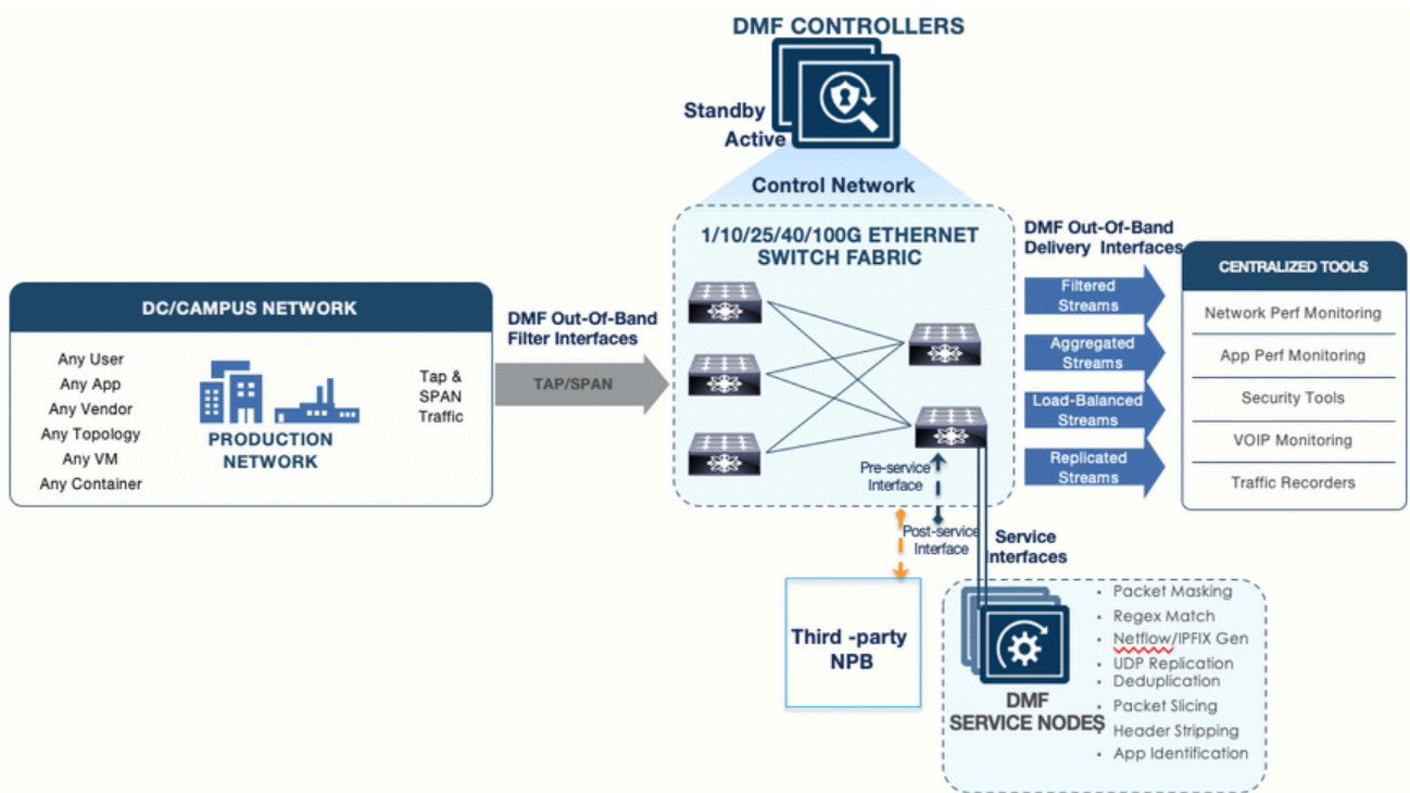
Figure 3-2: DANZ Monitoring Fabric (DMF) Two-Tier Topology
