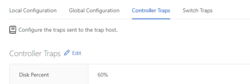
Figure 10-18: Disk Percent
