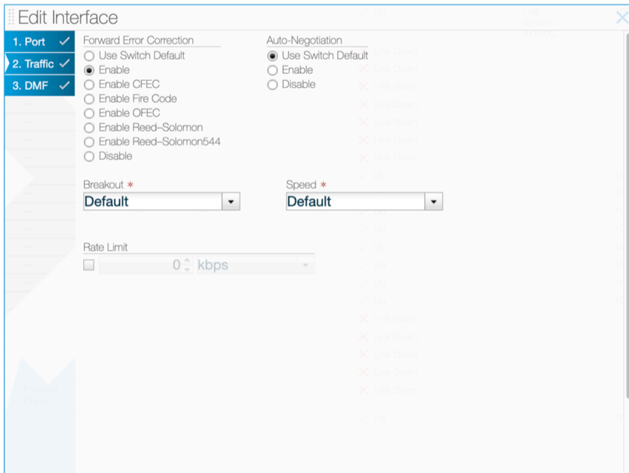
Figure 5-5: FEC Configuration
