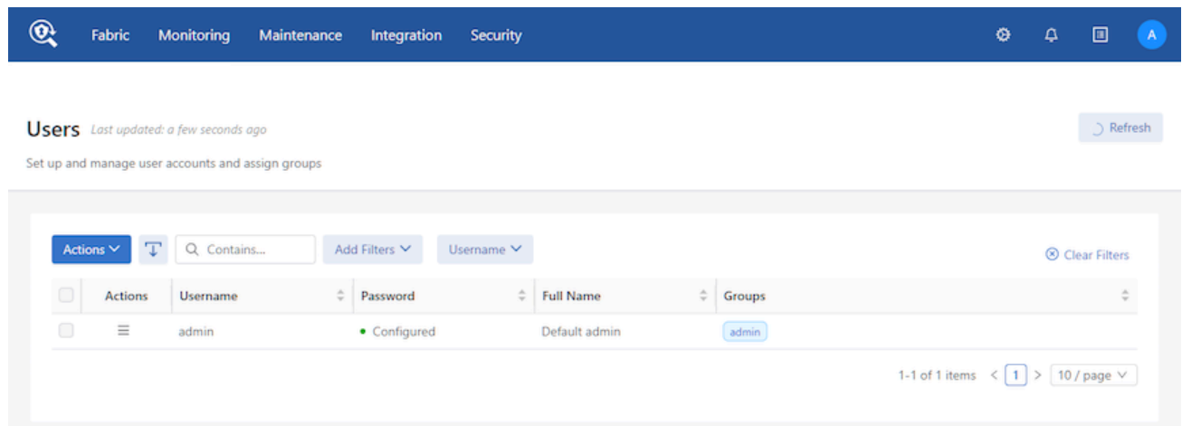
Figure 11-2: Security > Users
