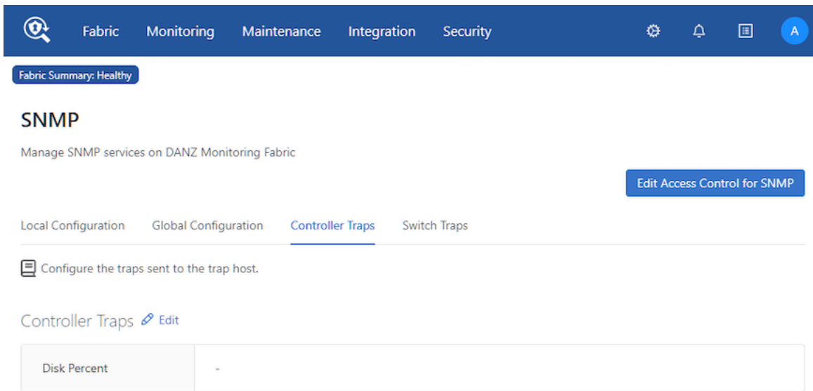
Figure 10-16: Controller Traps
