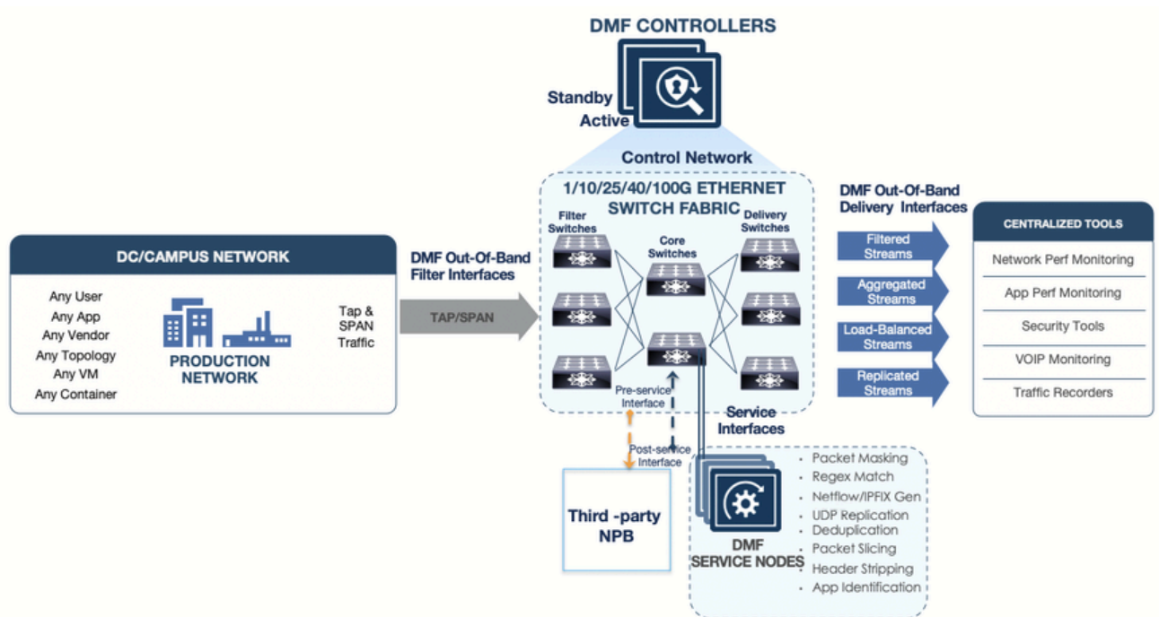
Figure 3-3: DANZ Monitoring Fabric (DMF) Three-Tier (Any-TAP-to-Any-Tool) Topology
