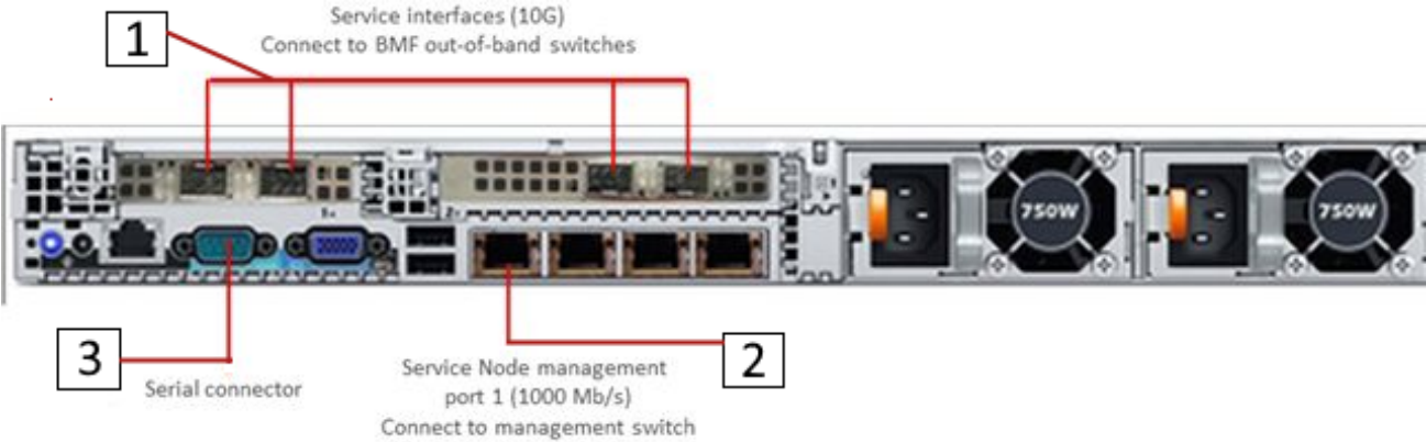
Figure 7-2: DMF Service Node (4-Port Appliance)
