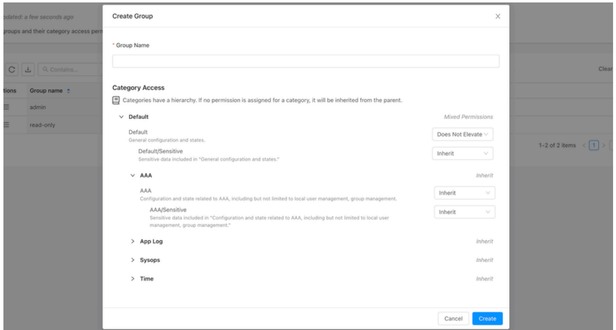
Figure 11-18: Custom Group
