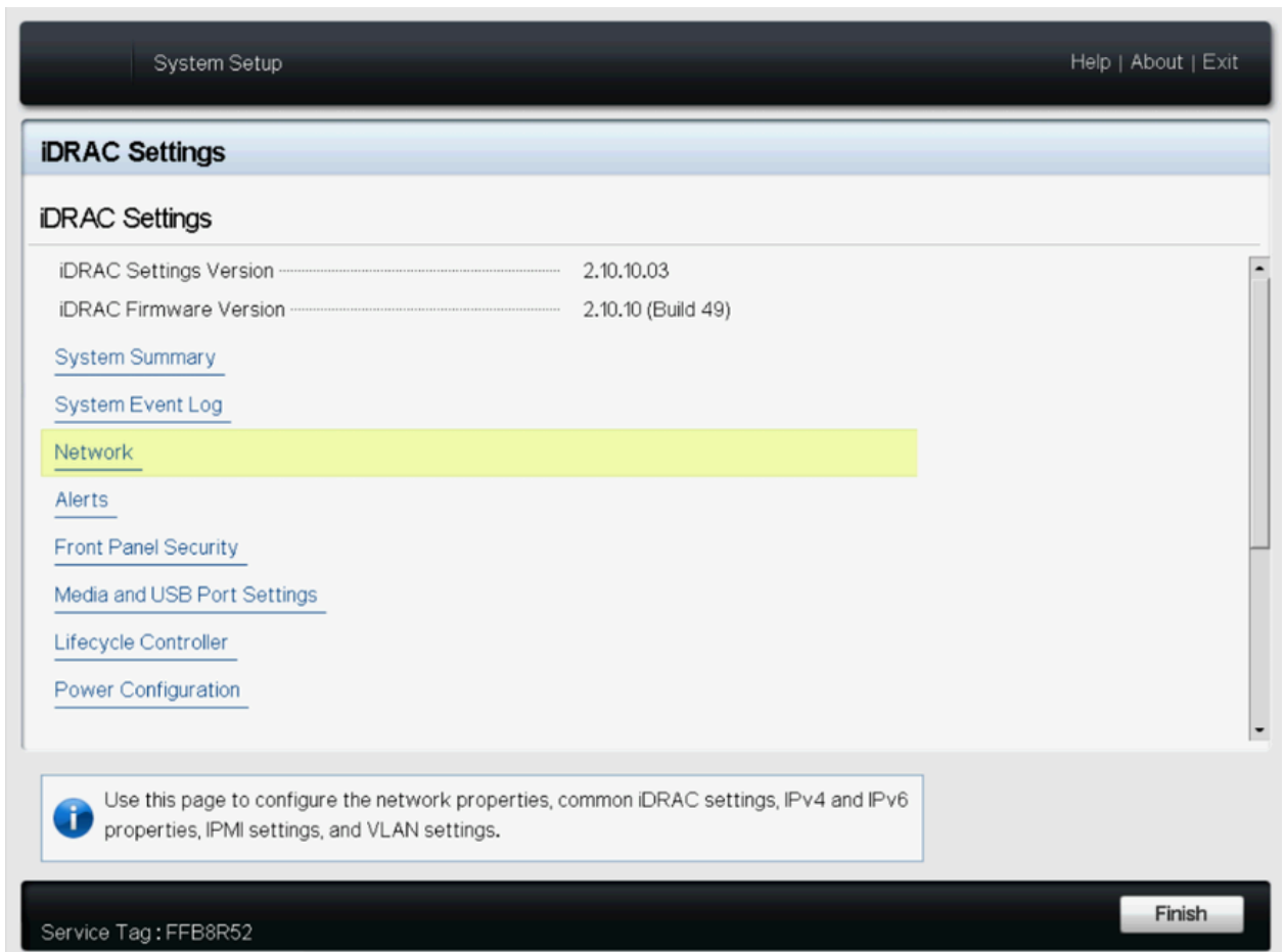
Figure 13-2: iDRAC Settings
