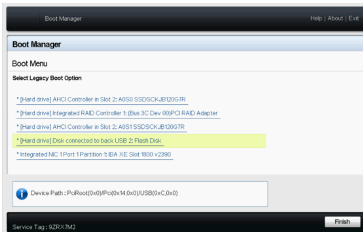
Figure 8-6: Boot Menu
