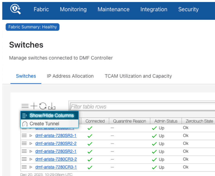
Figure 4-19: Show/Hide Columns
