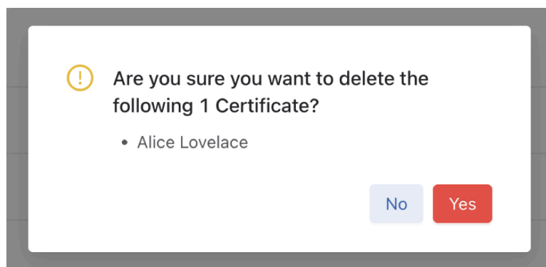
Figure 12-8: Confirmation Window
