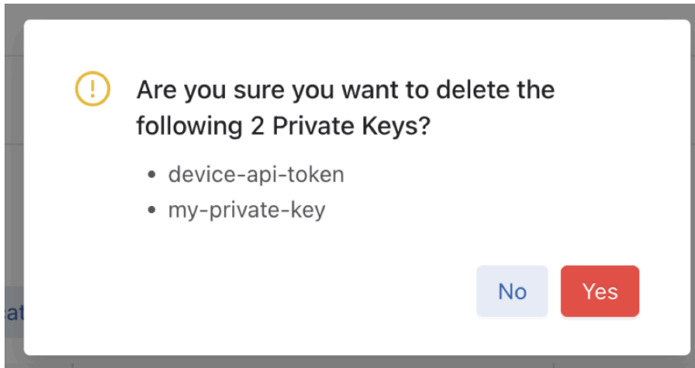
Figure 12-14: Confirmation Window
