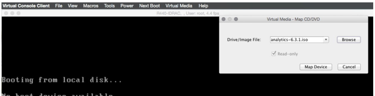
Figure 14-22: Map Device
